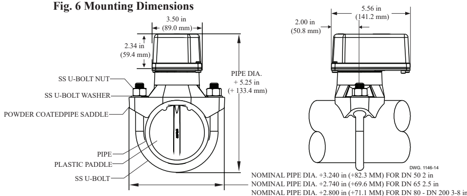
Fig. 6 Mounting Dimensions
