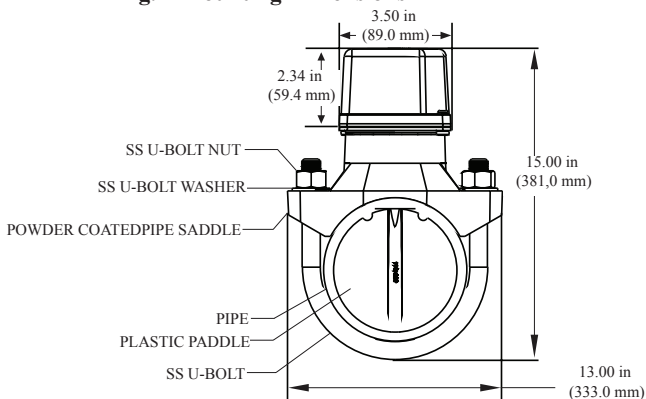
Fig. 7 Mounting Dimensions
