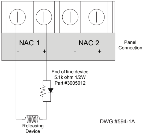
Figure 15. NAC Releasing Circuit Wiring with EOLD Assembly
