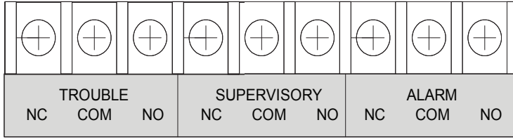
DWG #593-26
