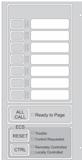
Figure 49. SB-8 Overlay
