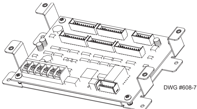
Figure 24. DRV-50 Board Showing Mounting Bracket
