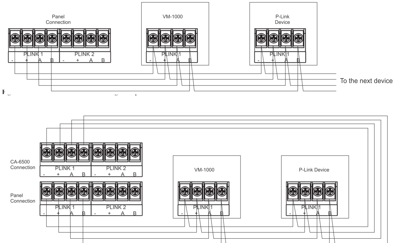
Figure 43. VM-1000 P-Link Class A Wiring Example
