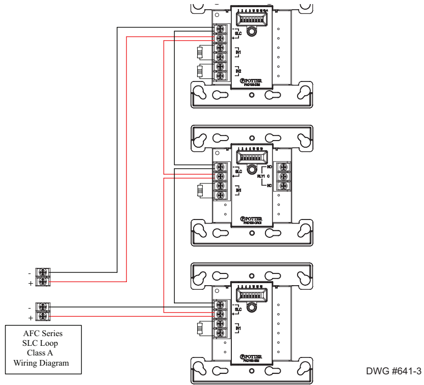
Figure 8. PAD Protocol Example of SLC as Class A
