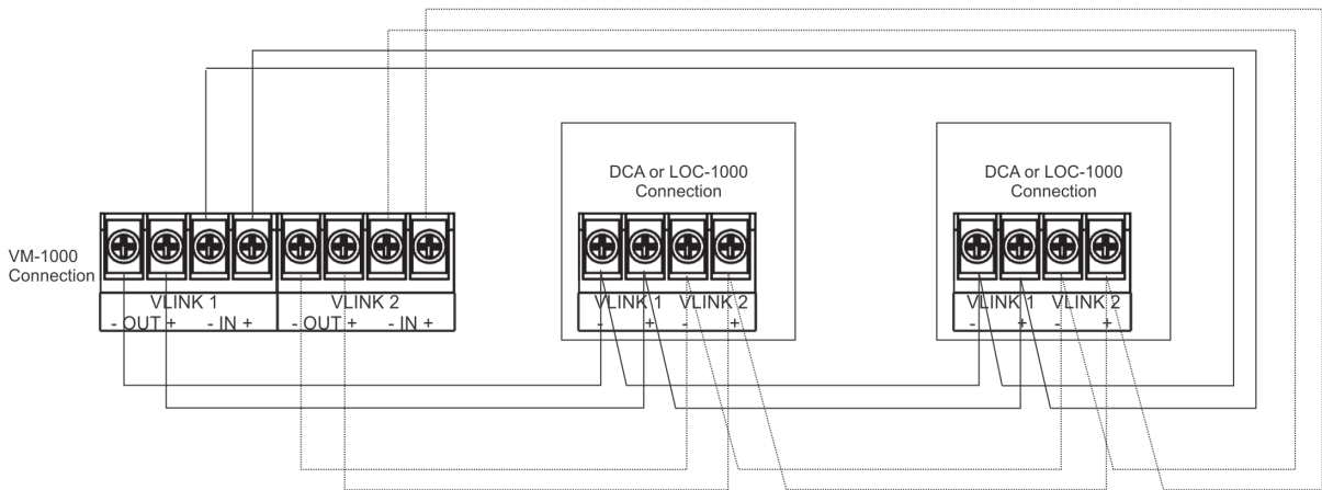
Figure 47. VM-1000 V-Link 1 and 2 Class A Wiring Example
