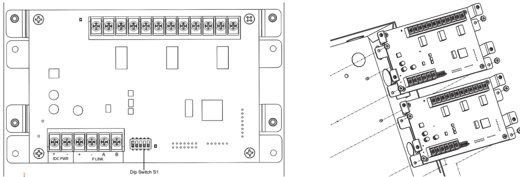
Figure 34. IDC-6 Initiating Device Circuit Expander and IDC-6 Installation
