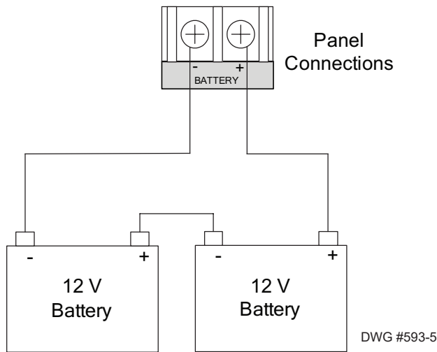
Figure 3. Battery Circuit Connections
