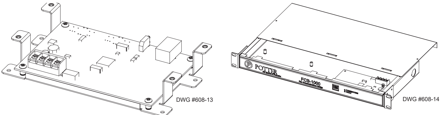
Figure 30. FCB-1000 Bridge & FCB-1000RM Showing Rack Mount
