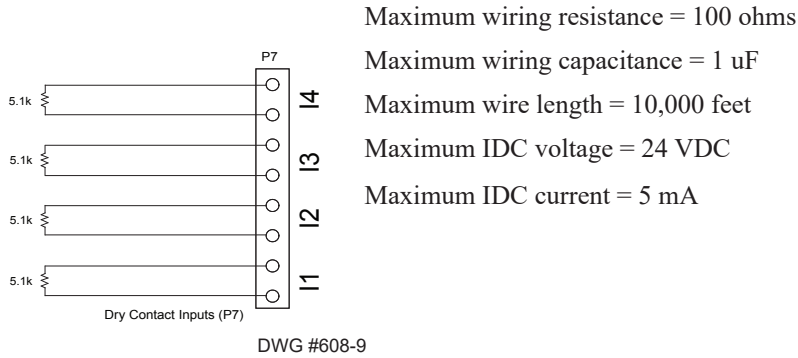
Figure 26. DRV-50 Dry Contact Input "P7" Connector
