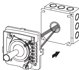
Step 2 Mount the back plate directly to the wall or to a 4" square box.
