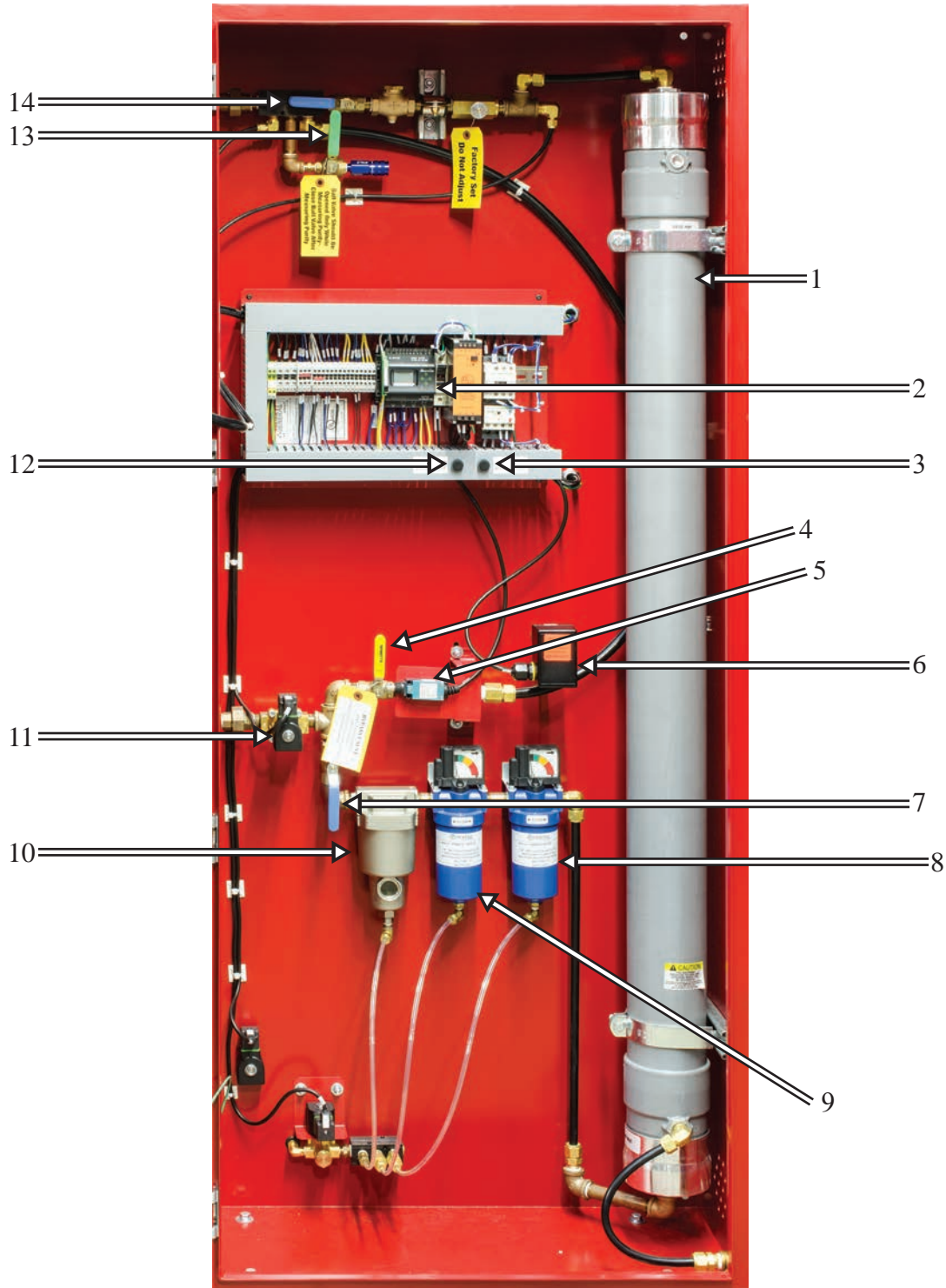
Figure 3: Typical NGP-2200D-M2/M3/M4/M5 Internal View
