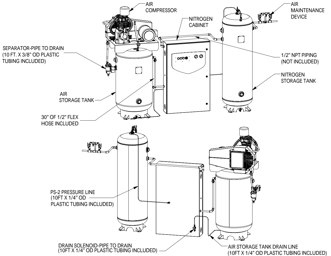
Figure 4: Piping Requirements
