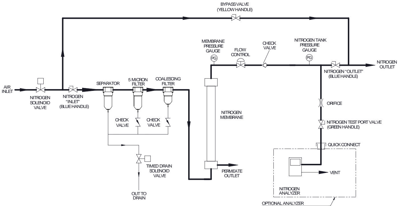
Figure 1: NGP-2200D-M2/M3/M4/M5 System Diagram
