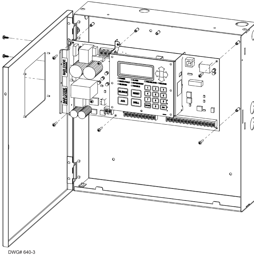
Figure 40. AFC-100 Cabinet Showing Circuit Board Assembly
