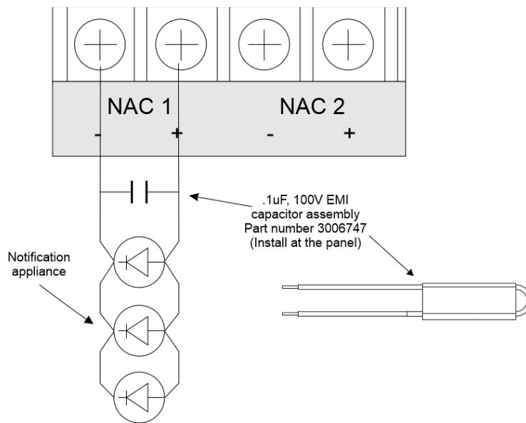
Figure 6. NAC EMI capacitor assembly wiring diagram
