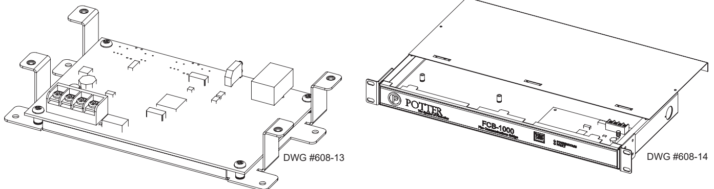
Figure 31. FCB-1000 Bridge & FCB-1000RM Showing Rack Mount
