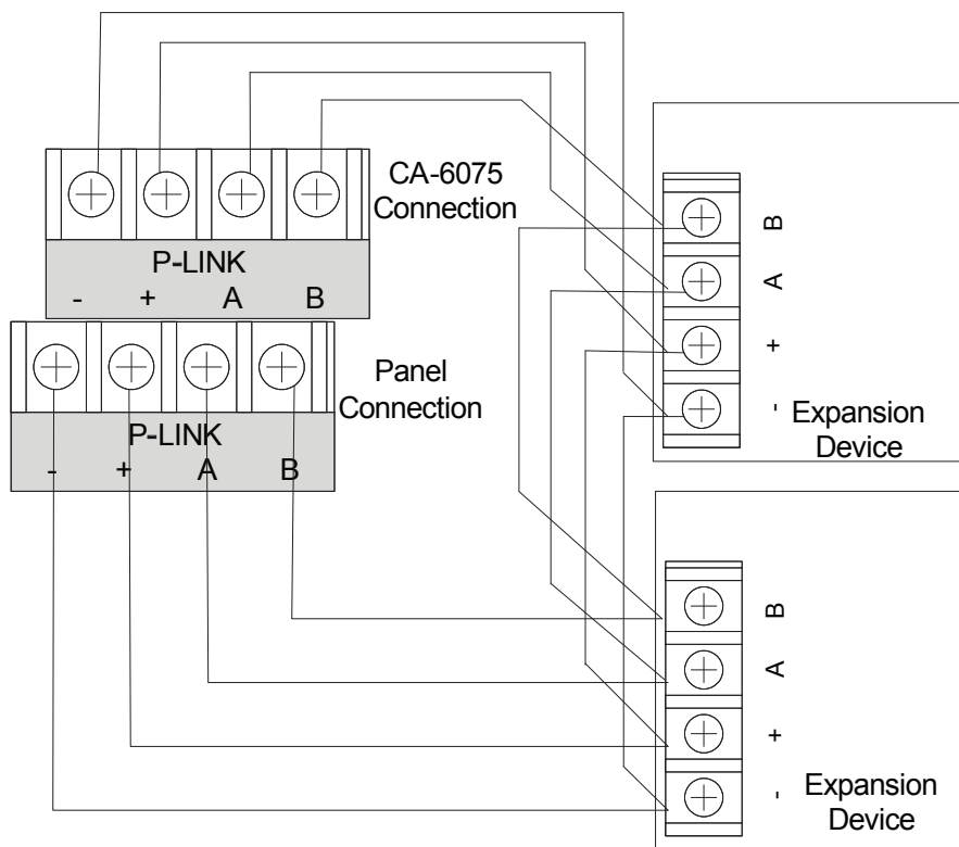
Figure 15. Example of P-Link Class A Wiring Requiring a CA-6075
