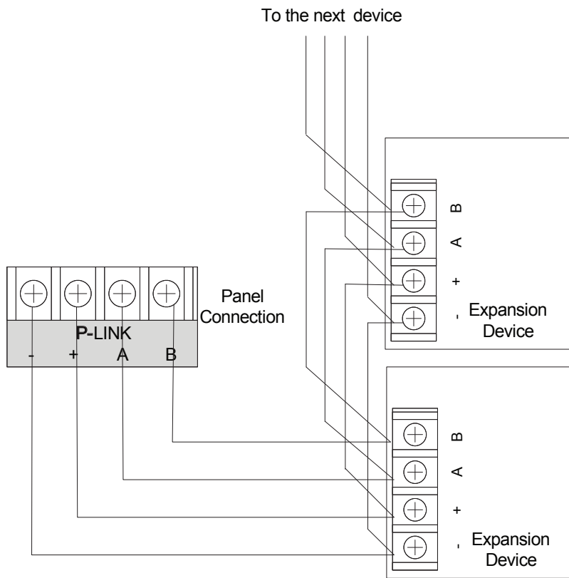
Figure 14. Example of P-Link Class B Wiring
