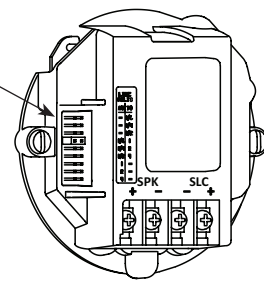
FIGURE 5: PAD100-SPKB Wiring and Power Tap
