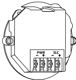
FIGURE 3: PAD100-LFSB Wiring
