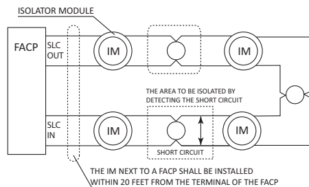
FIGURE 2: Wiring (Class X) Using PAD100-LFSB and PAD100-IM
