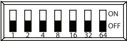
FIGURE 13: Enlarged View of PAD Device with Dip Switch Setting Unaddressed
