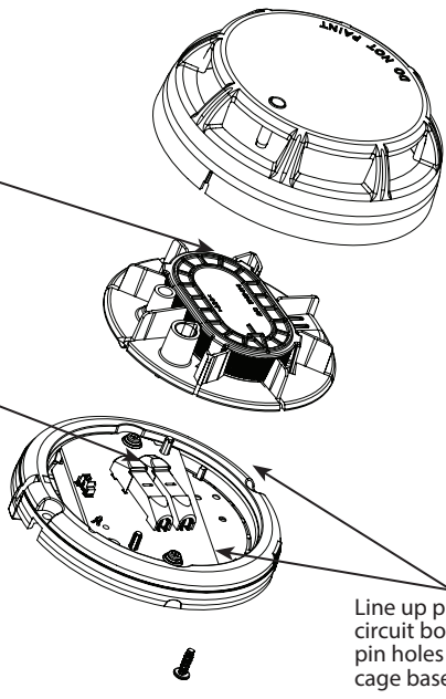
FIGURE 8: Remove Optic Cage Base from Detector for Cleaning (PD models only)
