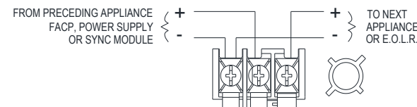
Figure 1: PE series 4X/3R STROBE
