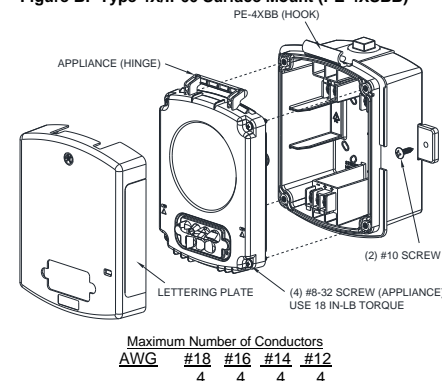
Figure B: Type 4X/IP66 Surface Mount (PE-4XSBB)**
