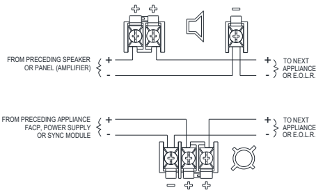
Figure 1: Speaker-Strobe (two circuits)
