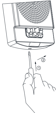
Figure 5: Grille Removal **
