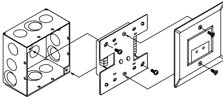
Figure 2: Installation into compatible electrical box
