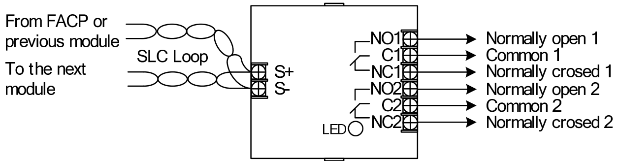
Figure 1: Wiring diagram of TRM-4
